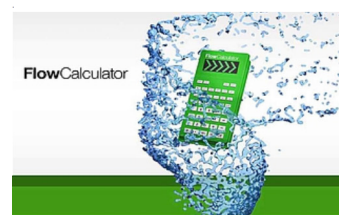
FlowCalculator preview
