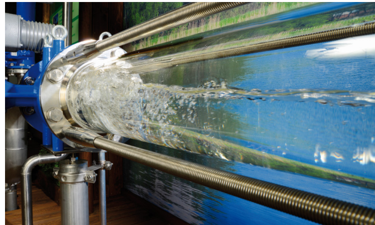
FlowCalculator preview
